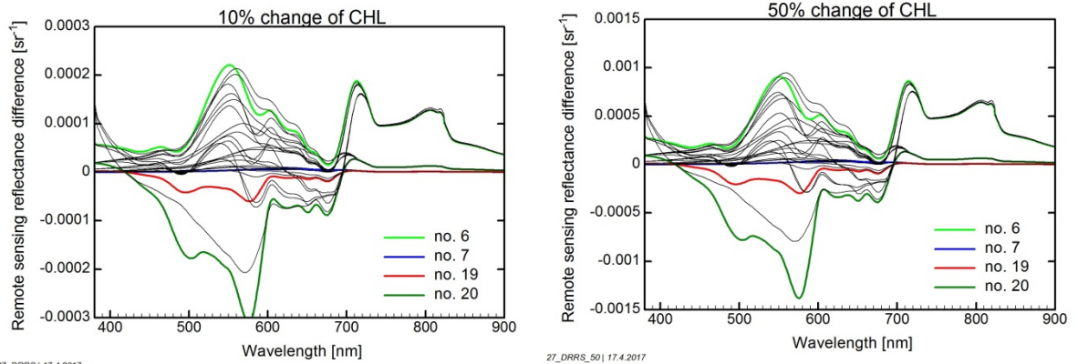
Figure 14: BOA remote sensing reflectance differences used to determine TOA radiance differences. The darkest spectrum (no. 7) induces the lowest change in reflectance, but the brightest spectrum (no. 19) not the highest. The highest reflectance differences are attributed to spectra no. 6 (in the NIR) and no. 20 (in the VIS).
