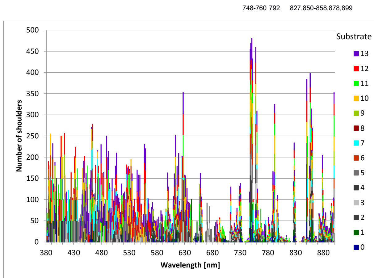
Figure 25: Cumulative histogram of the shoulders ( \partial^2 R_s / \partial \lambda^2 = 0 ) for very shallow water of 0.01 – 0.50 m depth.
