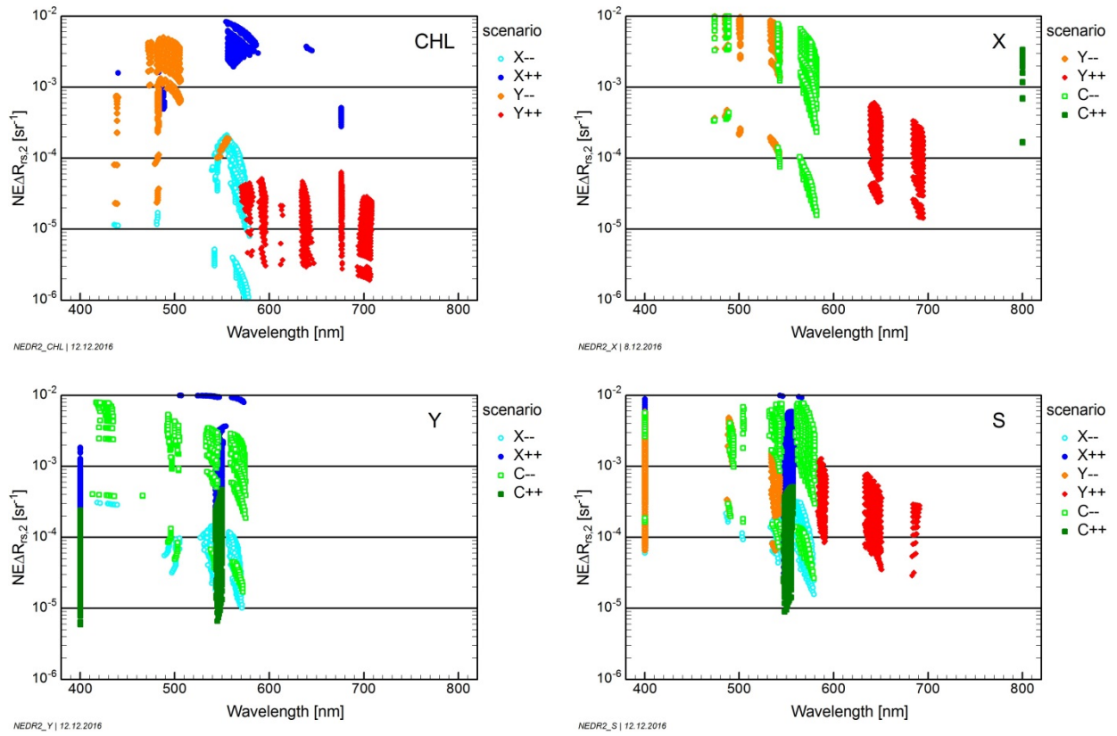
Figure 37: Maximum change of R_{rs} for a 10% change of the parameter indicated top right for the extreme scenarios.
