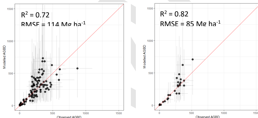
Figure 3.4 Comparison of observed and modelled aboveground biomass at 0.25 (left) and 1.0 (right) ha scales. The grey error bars represent 95% credible intervals in the LVIS predictions (y-axis) and the in situ estimates (x-axis).
