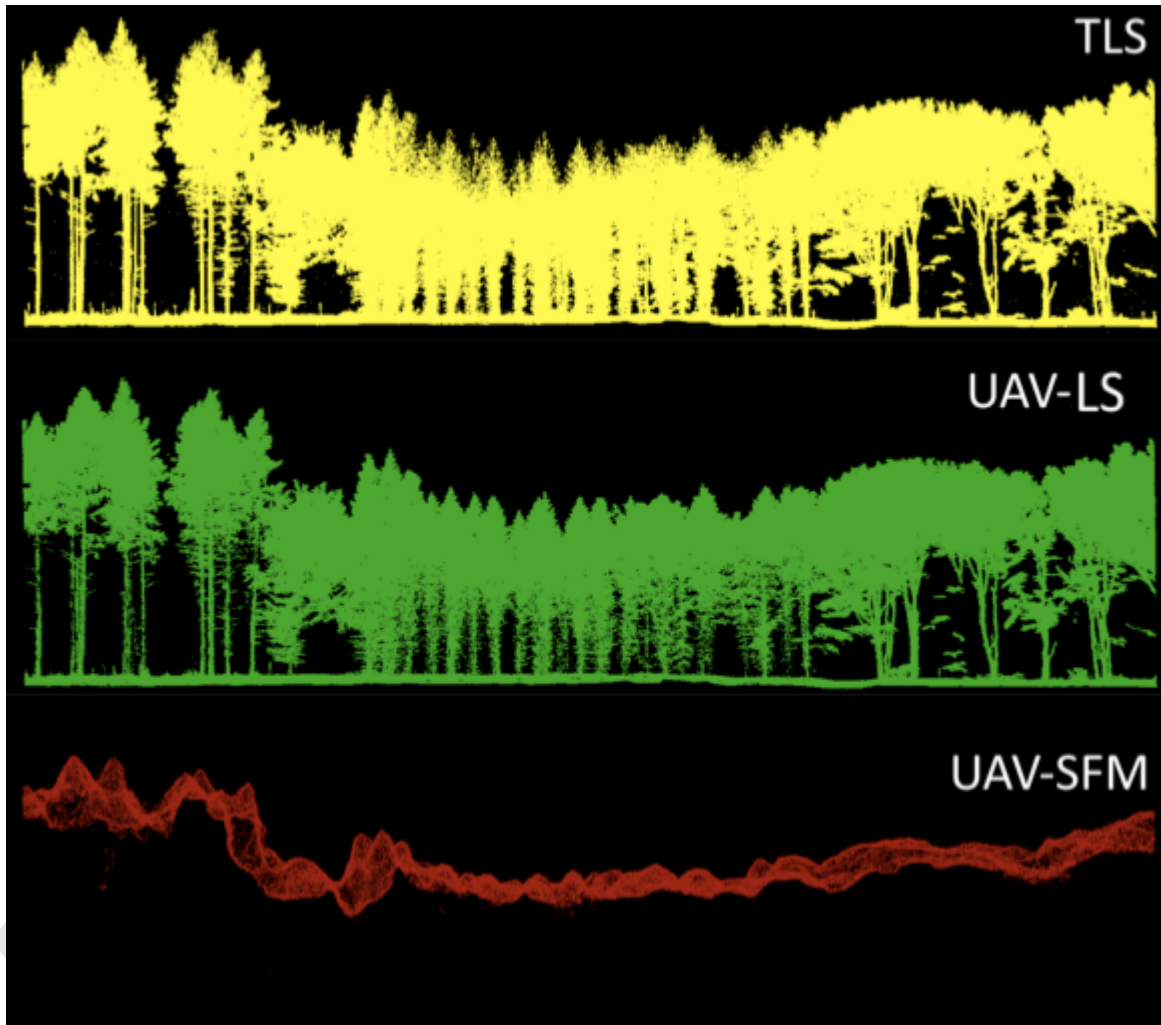
Figure 2.1 Slice of a forest with old Beech and Oak from the same perspective, acquired in the Netherlands with TLS (Riegl VZ-400)(top), UAV-LS (Riegl VUX-SYS) (middle) and UAV-SFM. The number of points in these slices are 69,547,639 (TLS); 5,396,682 (UAV-LS) and 96,229 (UAV-SFM)
