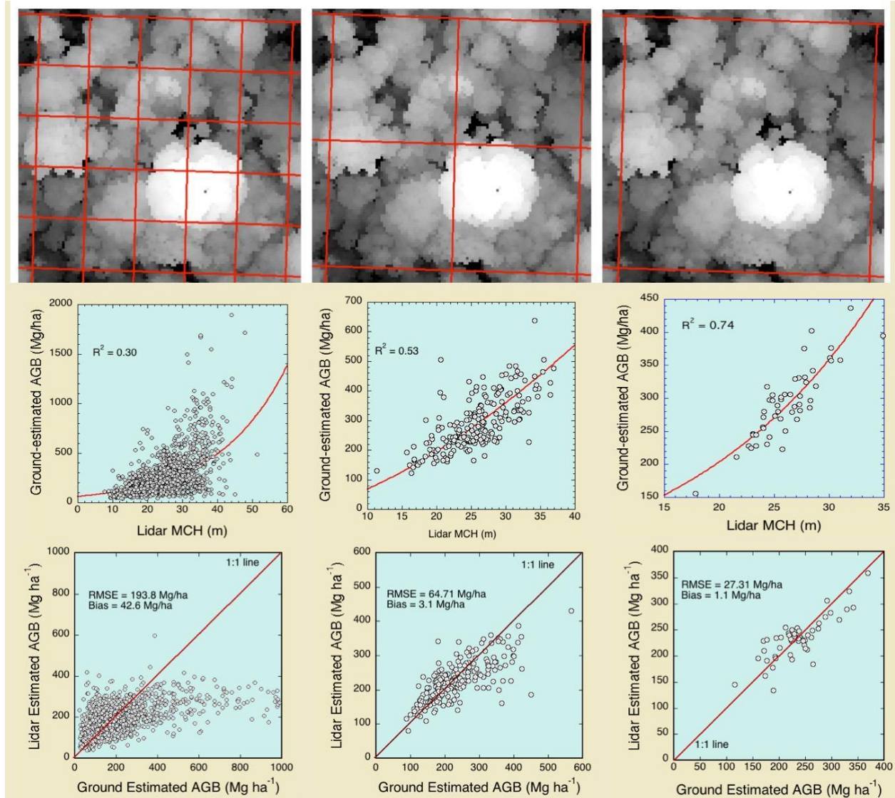
Figure 3.5 Ground plots of different size and lidar biomass models developed with mean top canopy height in tropical forests of Barro Colorado Island in Panama. The plots in the 1 m resolution Lidar data suggest that at scale of 20 m x 20 m (a), there is large bias in the model, but gradually at areas of 50 m x 50 m (b) and 100 m x 100 m ©, the model improves and the estimate of biomass can be made without significant bias.
