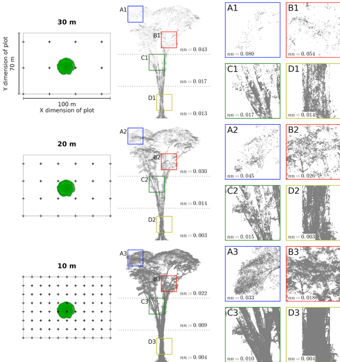
Figure 2.3 A comparison of mean nearest neighbour distance for points that comprise an individual tree derived using 10, 20 and 30 m grid sampling densities. (Left column) The location of sample points and location and extent of the target tree. (Middle column) Point cloud
